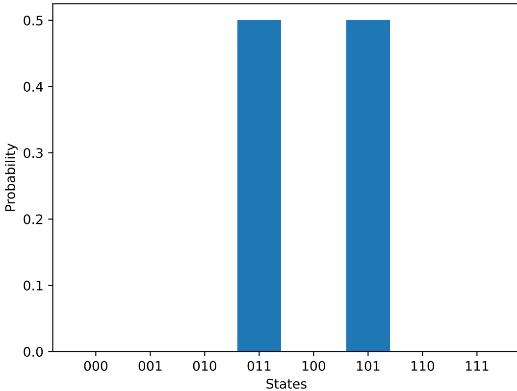
Grover Search Results (2 Targets)
