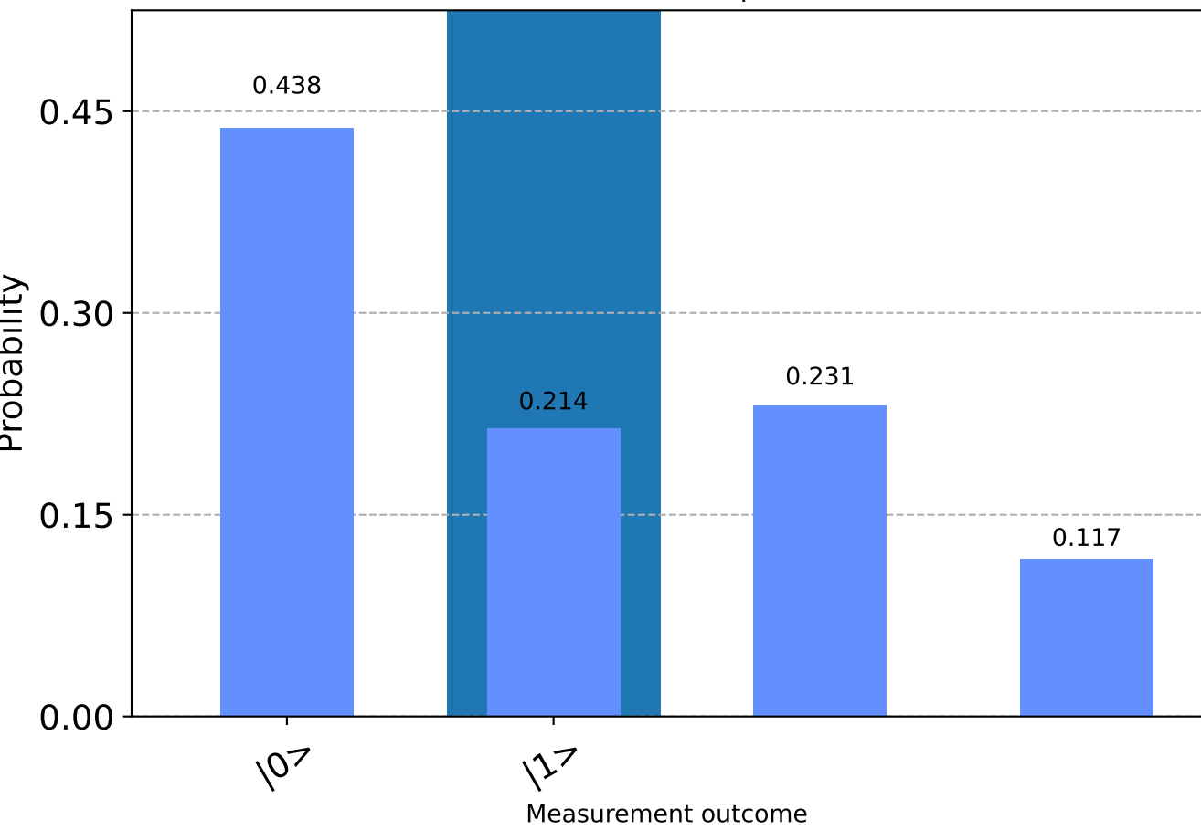
Measurement Outcomes after Optimisation. Cost: -1.0
